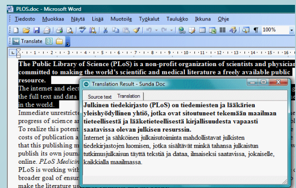
A pop-up window showing a text fragment translation.
